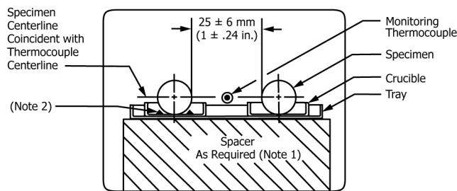
(b) Furnace Chamber—Cross Section View
