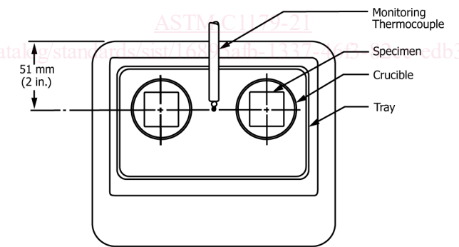
(a) Furnace Chamber—Top View
