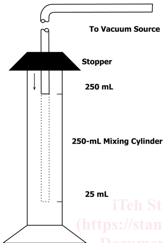
FIG. 1 Vacuum Apparatus
