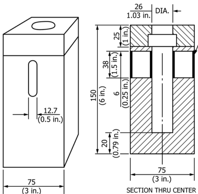
BALSA WOOD CELL CARRIER FIG. 4 An Example of an Insulated Cell Carrier
