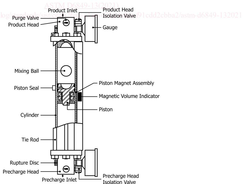
FIG. 1 Typical Floating Piston Cylinder (FPC)
