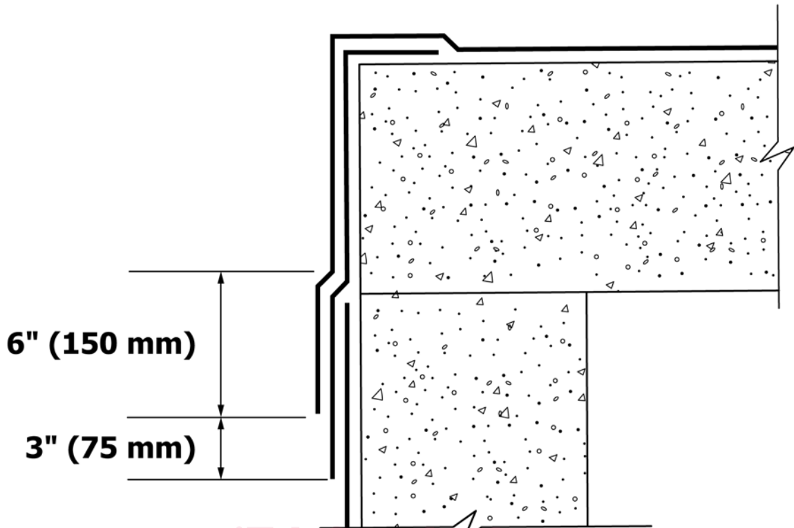
FIG. 8 Slab at Foundation
