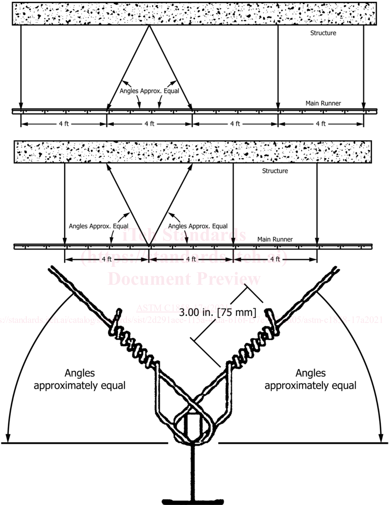
Method 3 - Countersplay Out-of-Vertical-Plane of the Main Runner
