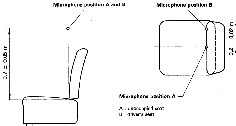
Figure — Microphone position with respect to a seat
