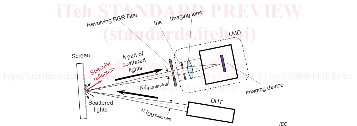
Figure 29 – Example of measurement geometries for colour speckle using an LMD with BGR filters
