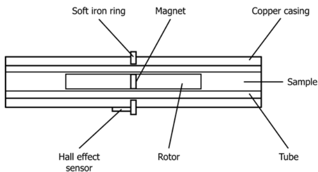
FIG. 1 Viscosity Cell
