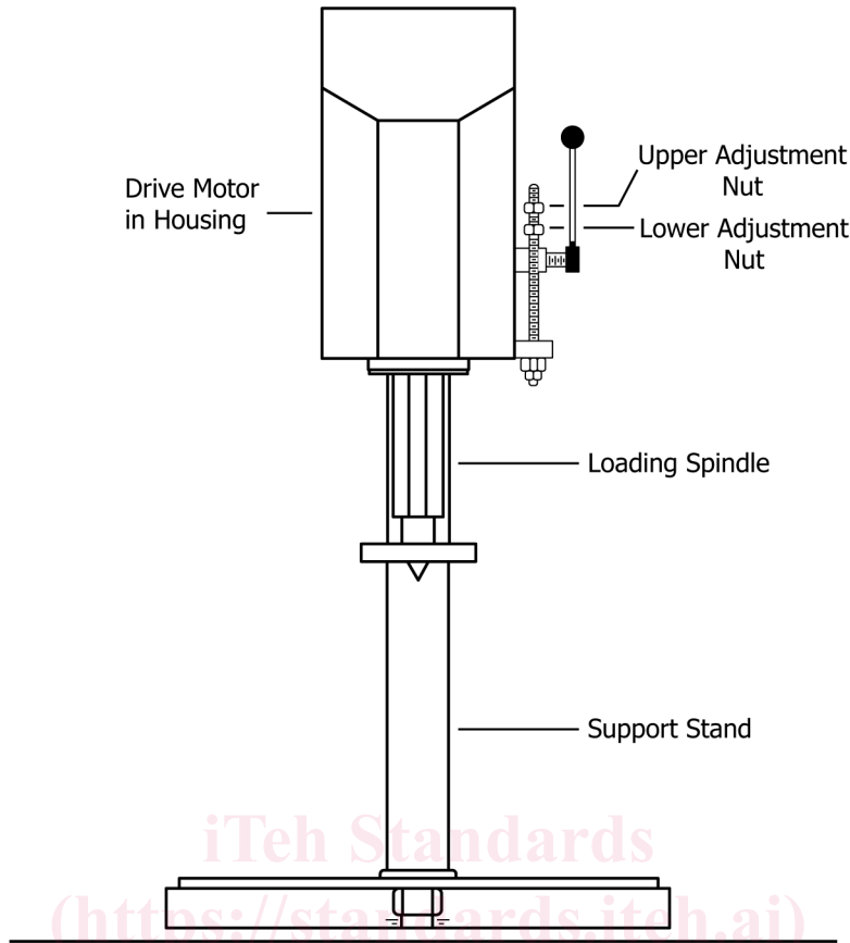
FIG. 3 Run-in Stand Drawing
