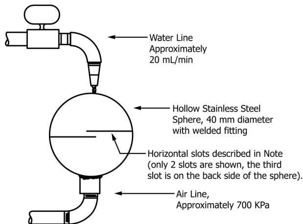
FIG. 1 Example of a Fog Spray for Maintaining Relative Humidity in Moist Rooms (Full Scale)
