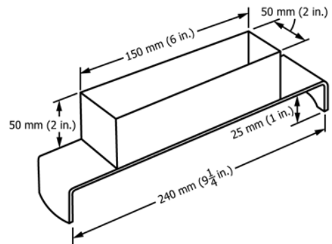
FIG. 1 Container for Early Stiffening Tests
