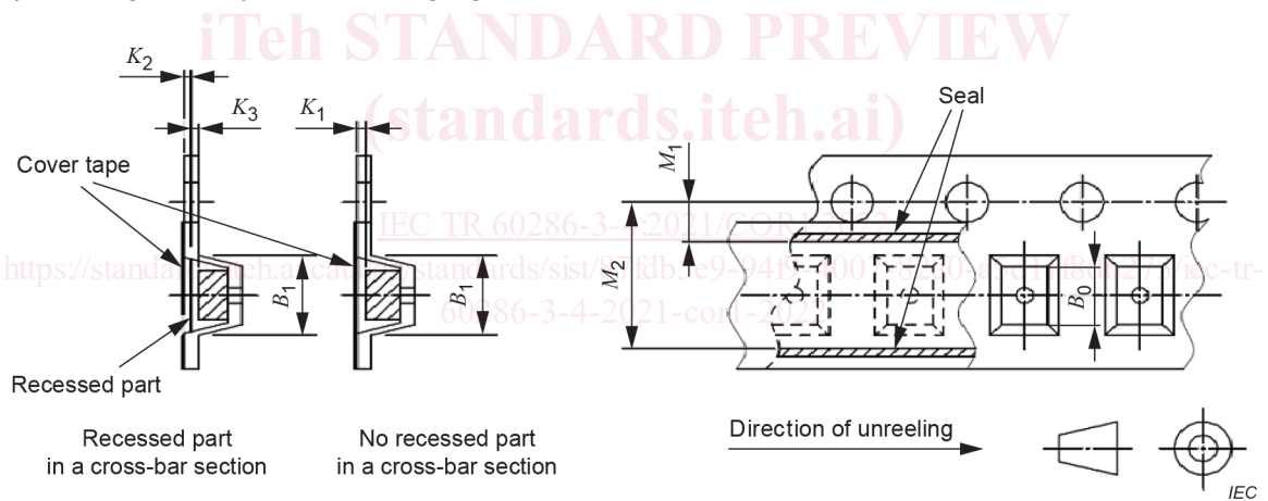
Figure 1 – Specified dimensions for emboss taping for Auto Loading Feeder
