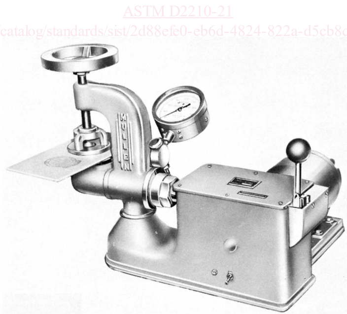
FIG. 1 Mullen Tester, Model A
