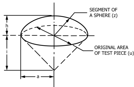
FIG. A1.1 Geometry for Derivation of Equation for Percentage Stretch
