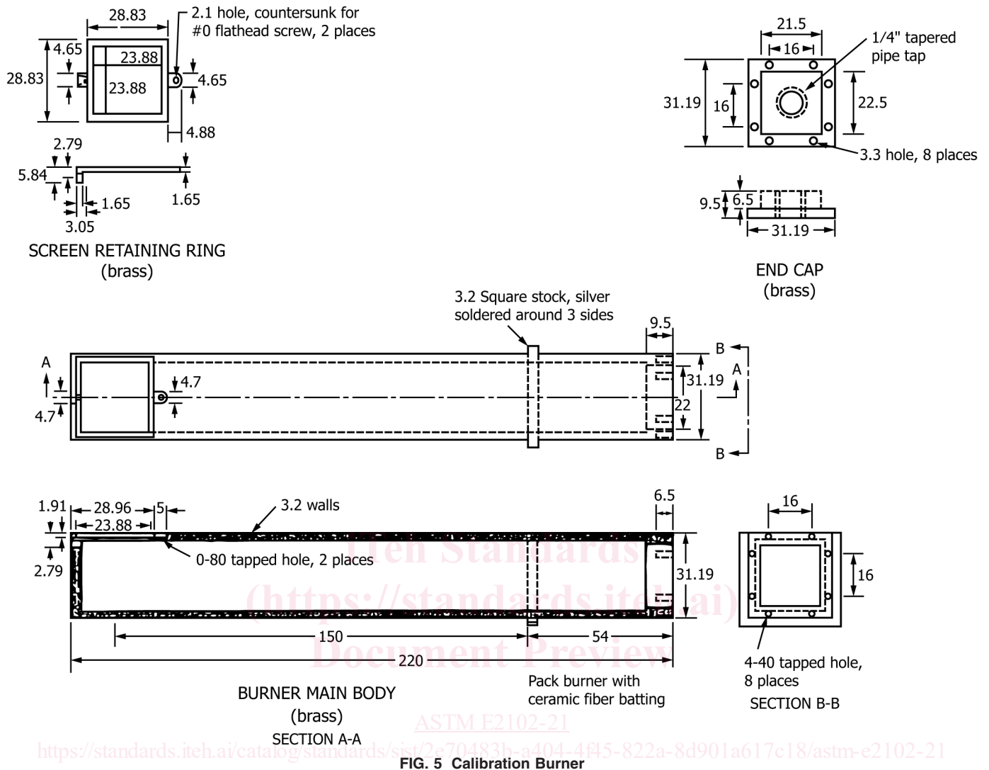
FIG. 5 Calibration Burner
