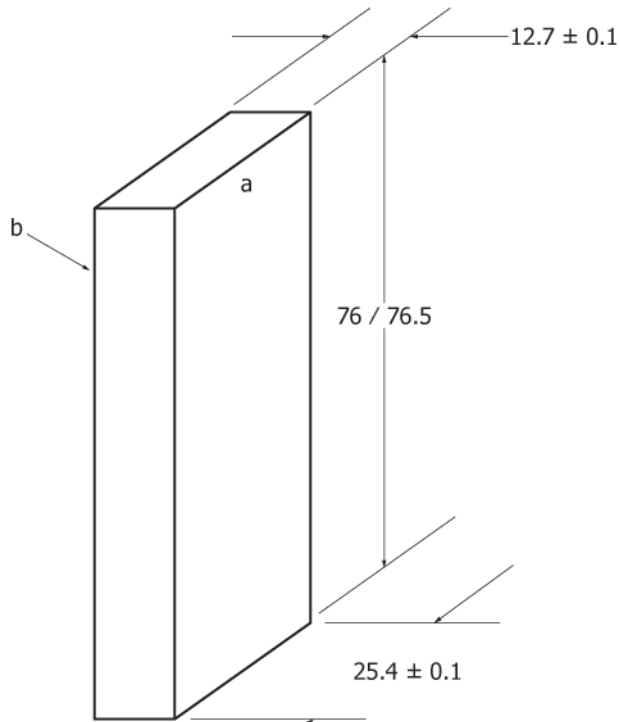
FIG. 2 Test Specimen Dimensions
