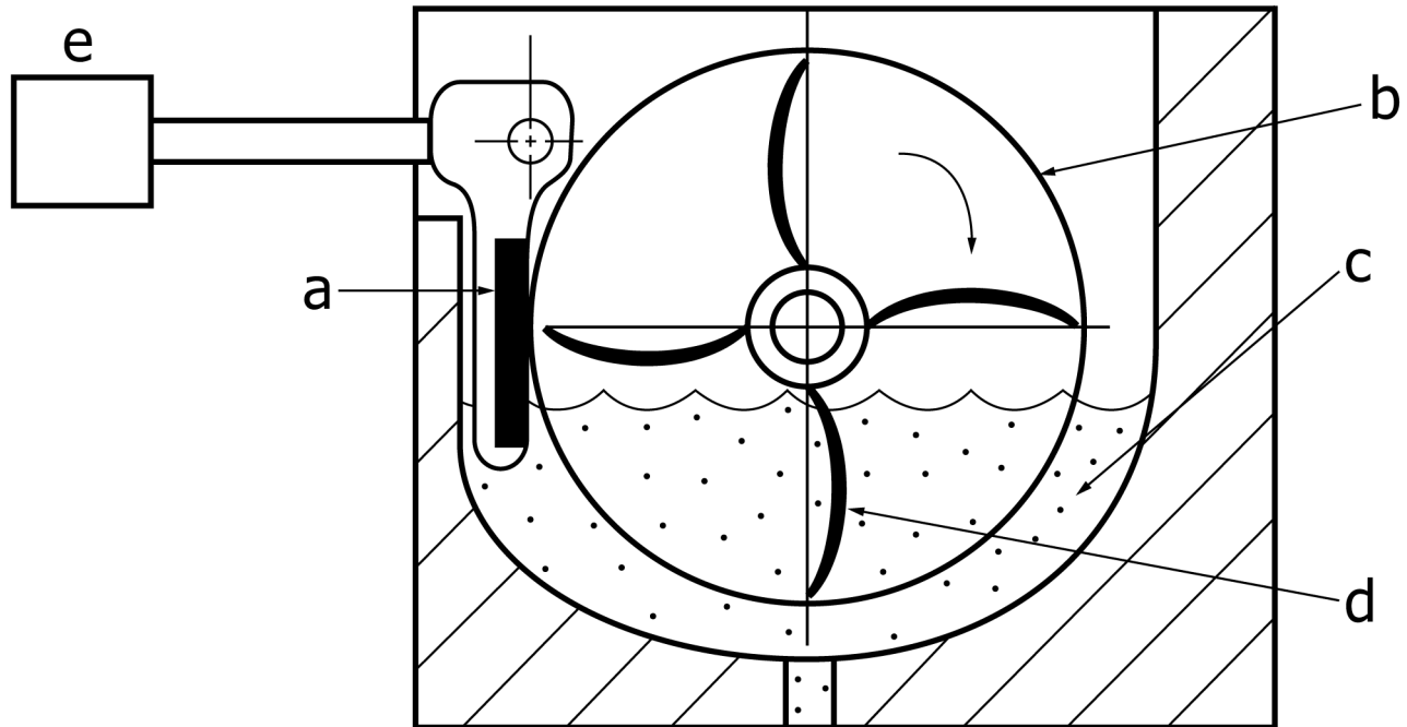
FIG. 1 Schematic of Test Rig
