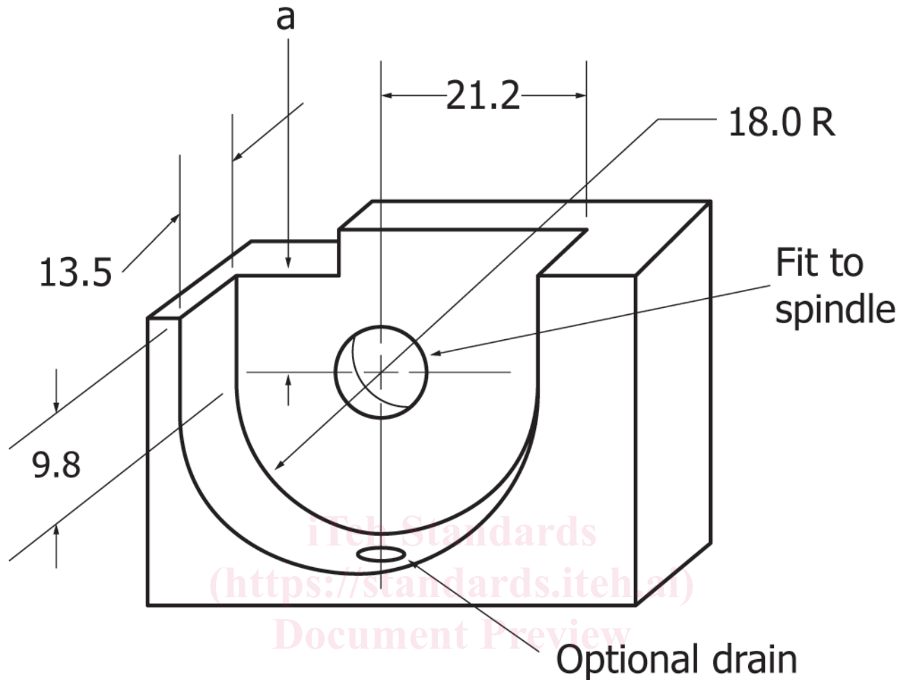
FIG. 3 Slurry Vessel
