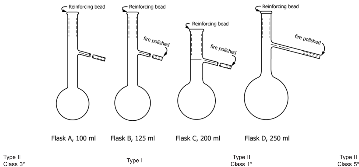
FIG. 3 Distillation Flasks
