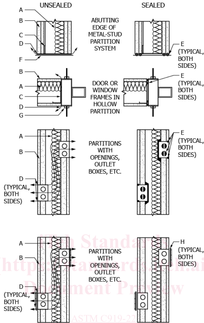
ARROWS SHOW SOUND TRAVEL PATH AROUND OR THROUGH PARTITIONS.
