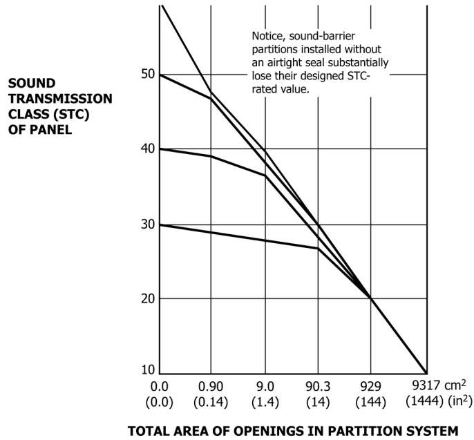
FIG. 2 Effect of Unsealed Hole Openings on STC-Rated Test Wall, 3.8 by 2.4 m (12 ft 6 in. by 8 ft) 3.8 m by 2.4 m (12 ft 6 in. by 8 ft)
