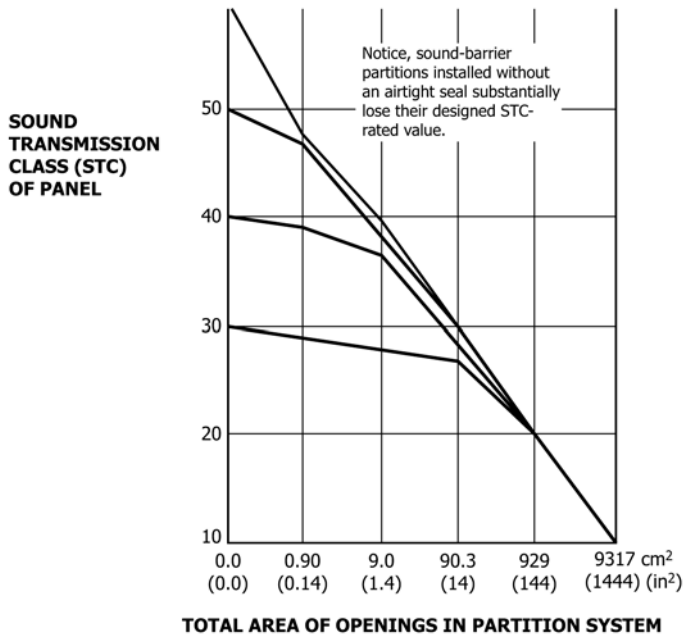
FIG. 2 Effect of Unsealed Hole Openings on STC-Rated Test Wall, 3.8 m by 2.4 m (12 ft 6 in. by 8 ft)
