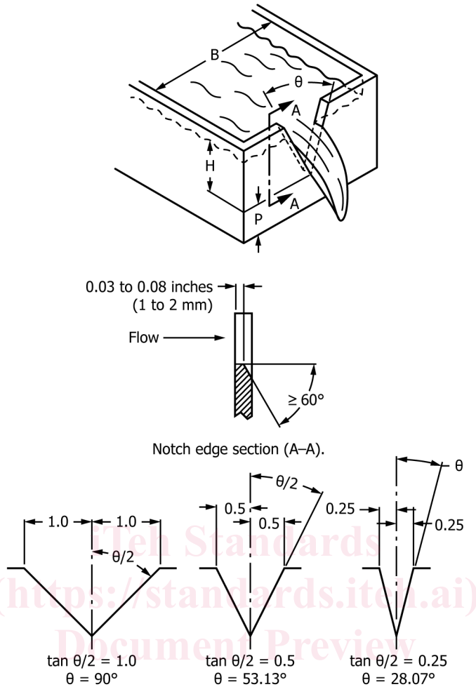
FIG. 4 Triangular Weirs
