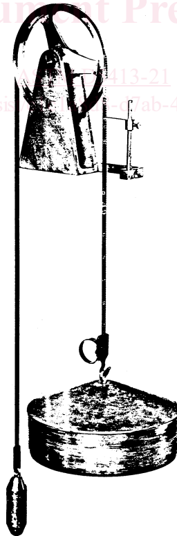
FIG. 4 Float-Type Gauge
