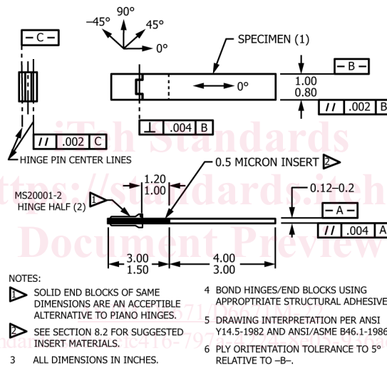
FIG. 7 Specimen—MMB Test (Inch-Pound Units)
