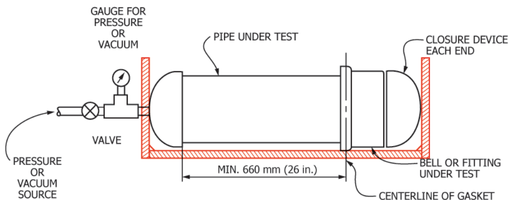
FIG. 1 Test Specimen
