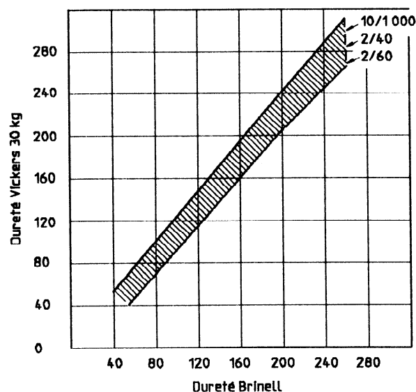
Figure B.2 — Conversion Vickers 30 kg — Brinell
