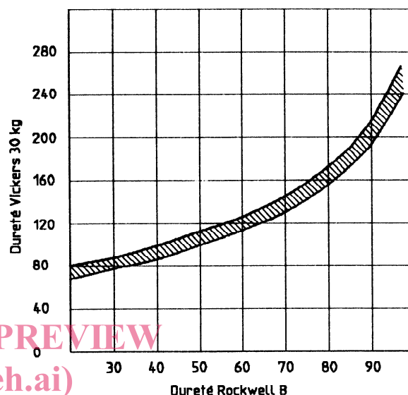
Figure B.1 — Conversion Vickers 30 kg — Rockwell B
