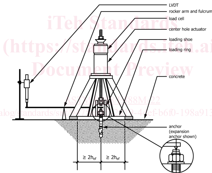
FIG. 2 Example of Unconfined Tension Test Setup – Displacement Measurement from top of Anchor
