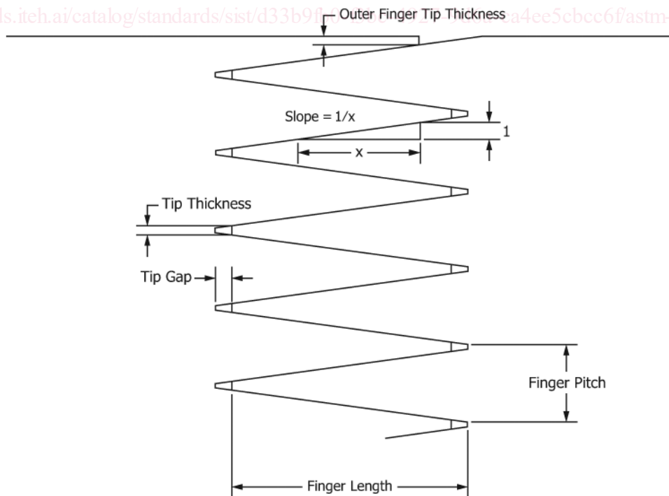
FIG. 1 Finger Joint Profile
