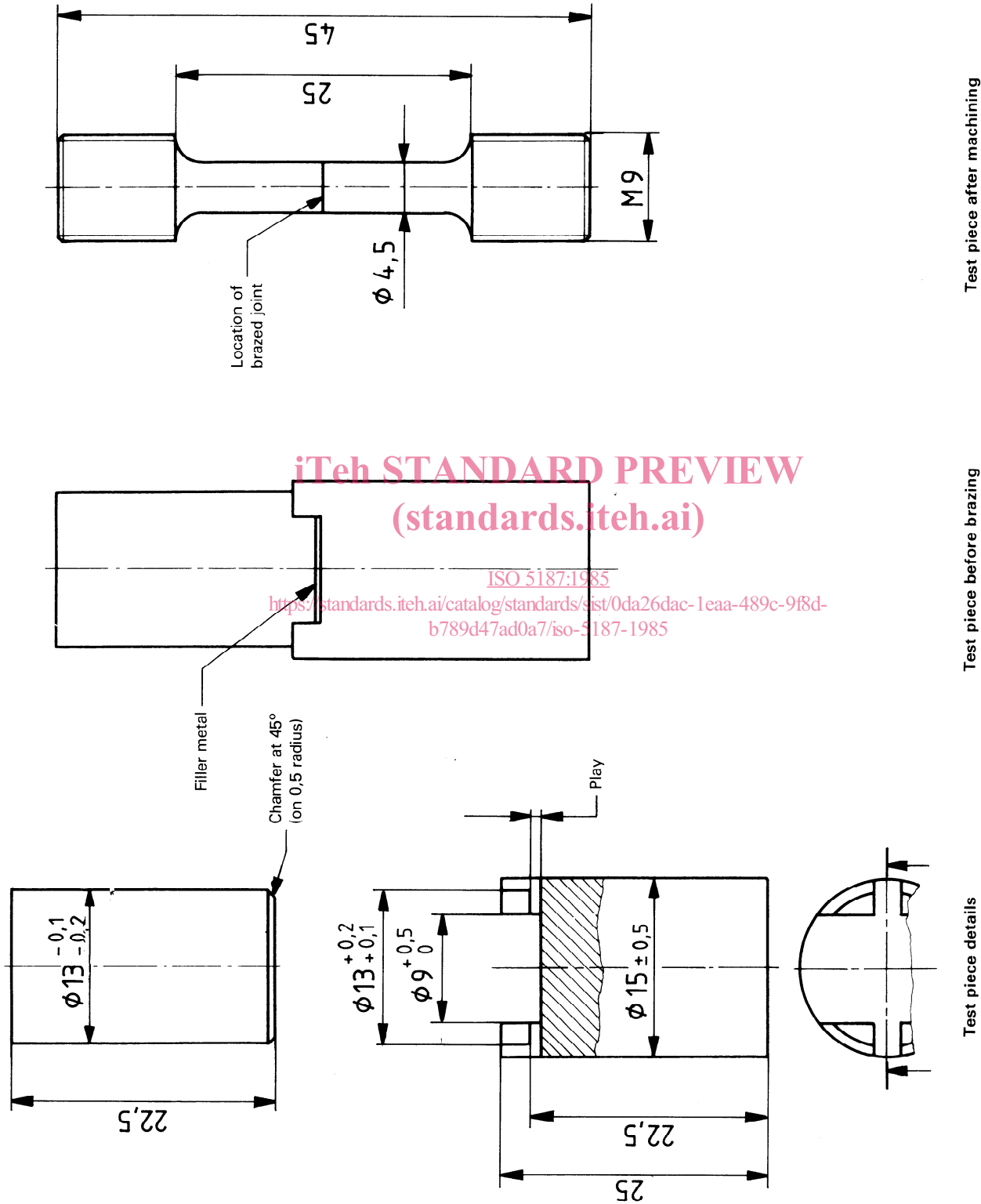
Figure 3 — Tensile test piece dimensions
