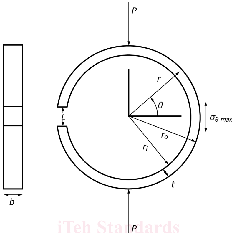
FIG. 1 —C-Ring-C-Ring Test Geometry with Defining Geometry and Reference Angle ( \theta ) for the Point of Fracture Initiation on the Circumference
