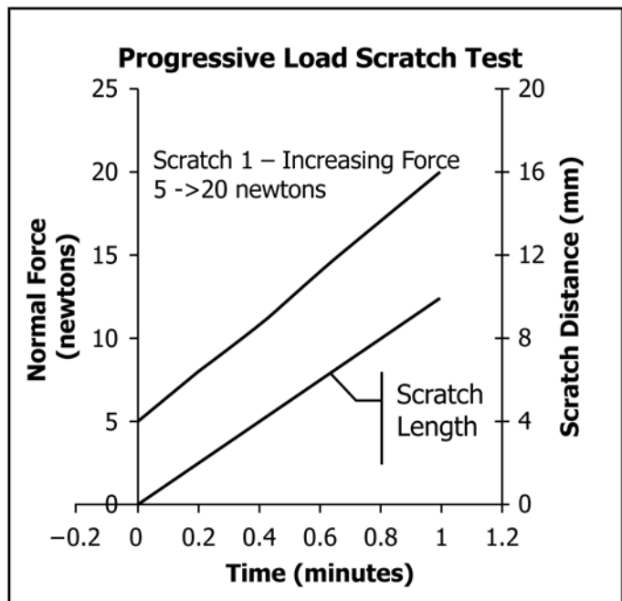
FIG. 4 Progressive Load Graph
