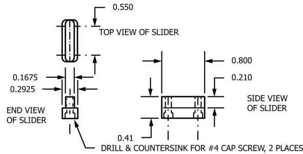
FIG. 15 Slider and Block for Connecting Pressure Block and Base Plate with Allowance for Opening Fixture
