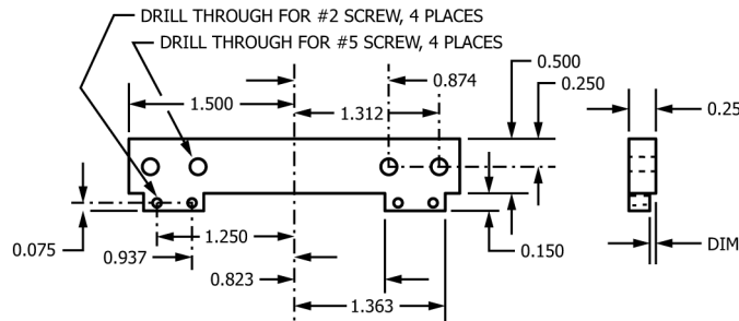
FIG. 11 Detail of Supplied End Launcher Body Adapted by Boring Out Tapped Holes
