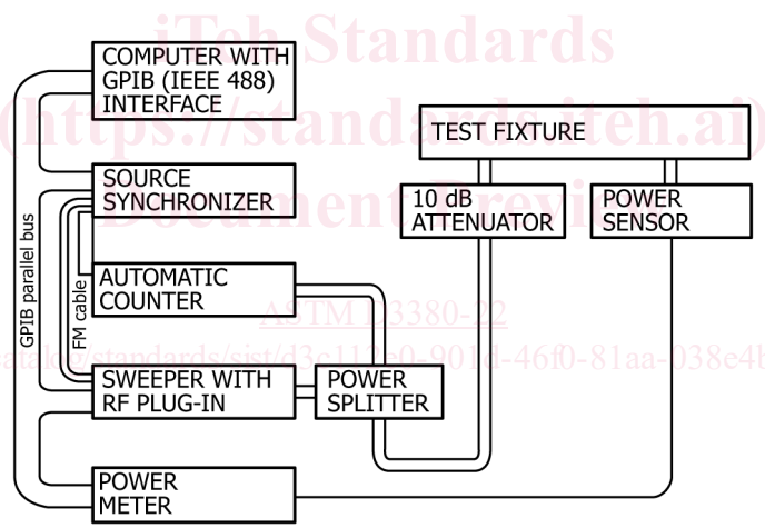
FIG. 17 Automated Permittivity Test Setup
