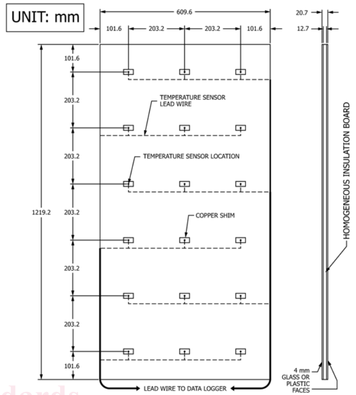
FIG. 2 (a) Example Calibration Transfer Standard Design Information
