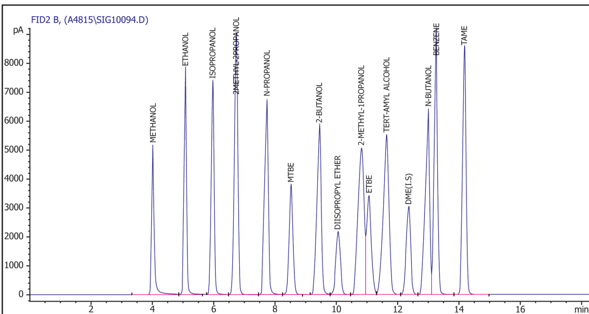
FIG. 1 Analysis of Oxygenates in Gasoline Schematic of Chromatographic System Example Chromatogram Showing Oxygenates
