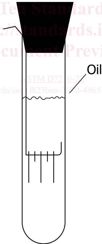
FIG. 2 Test Tube Arrangement
