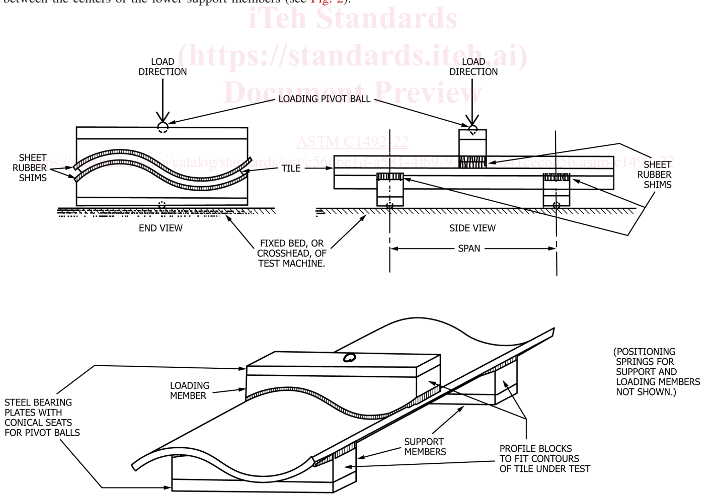
FIG. 2 Schematic of Assembly for Flexure Strength Testing
