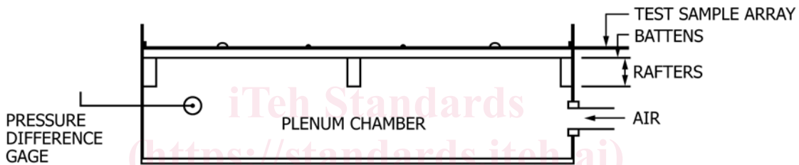
FIG. 2 Plenum Chamber Arrangement for Air Permeability Test
