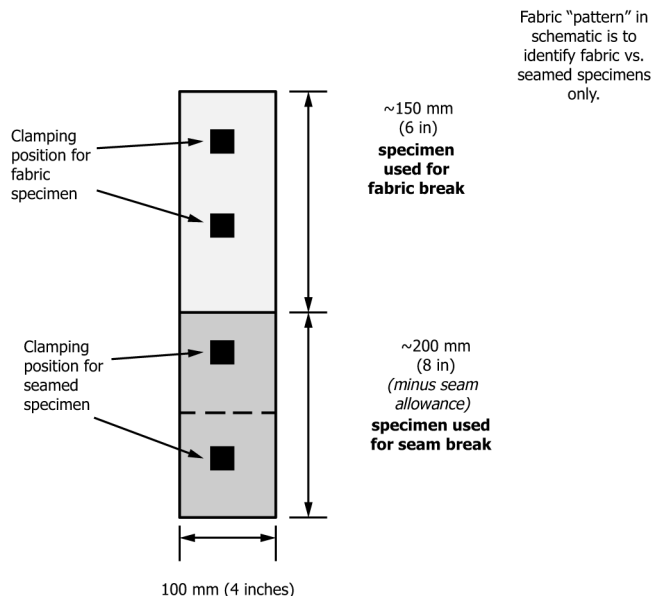
FIG. 4 Seamed Specimen Removed from Manufactured Item
