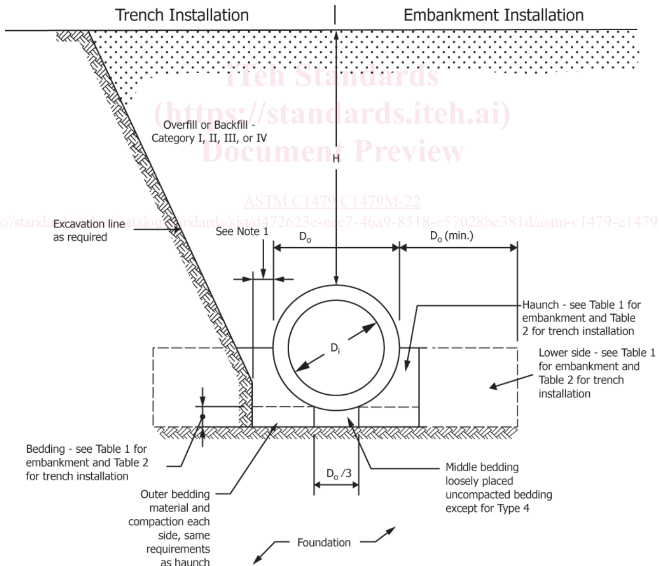
FIG. 2 Round Pipe Standard Embankment/Trench/Embankment Installations
