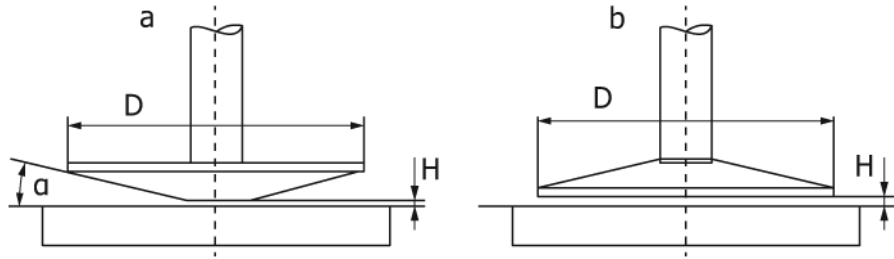
FIG. 1 Schematic Diagram of Cone-and-Plate (a) and Parallel Plate (b) Fixtures Geometries
