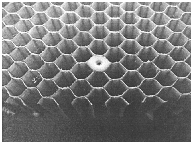
FIG. 2 Potted Honeycomb Cell
