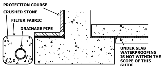
FIG. 1 Footing
