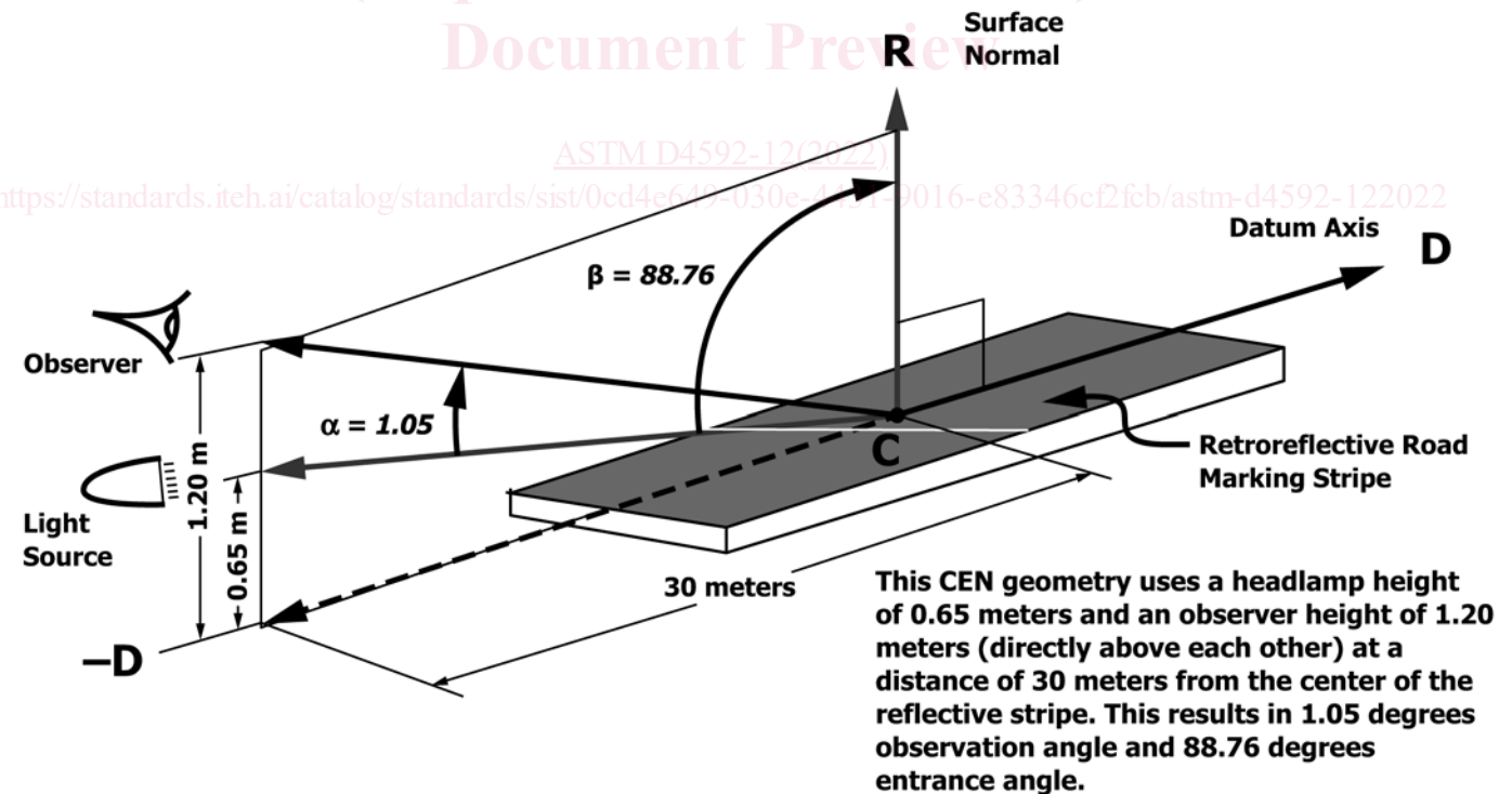
FIG. X1.1 CEN 30-Metre Geometry
