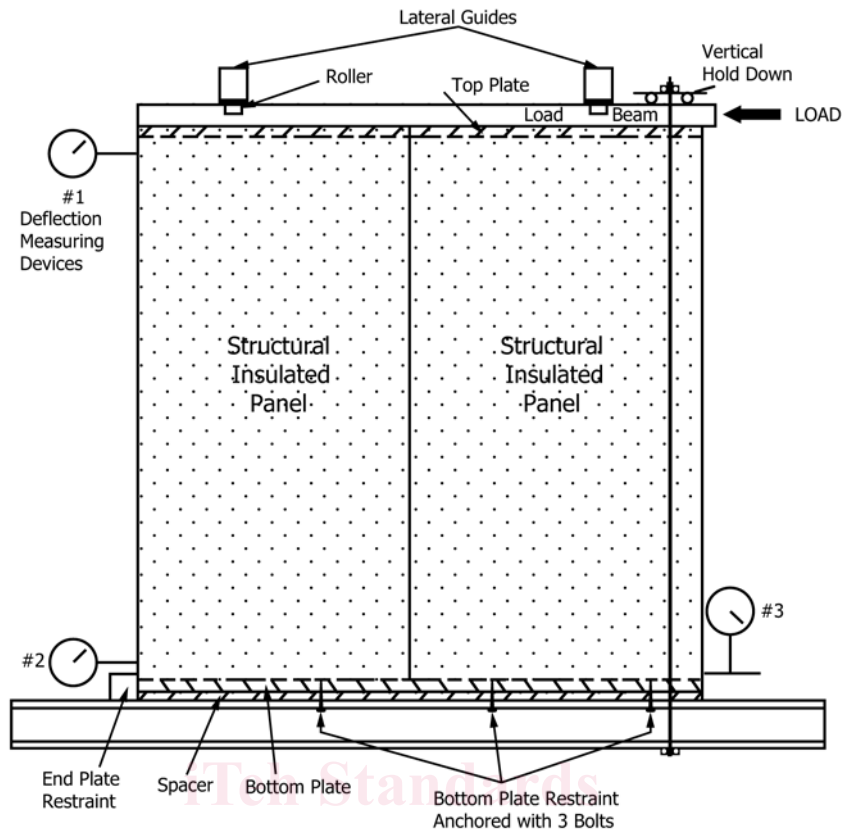
FIG. 2 Racking Load Test Assembly
