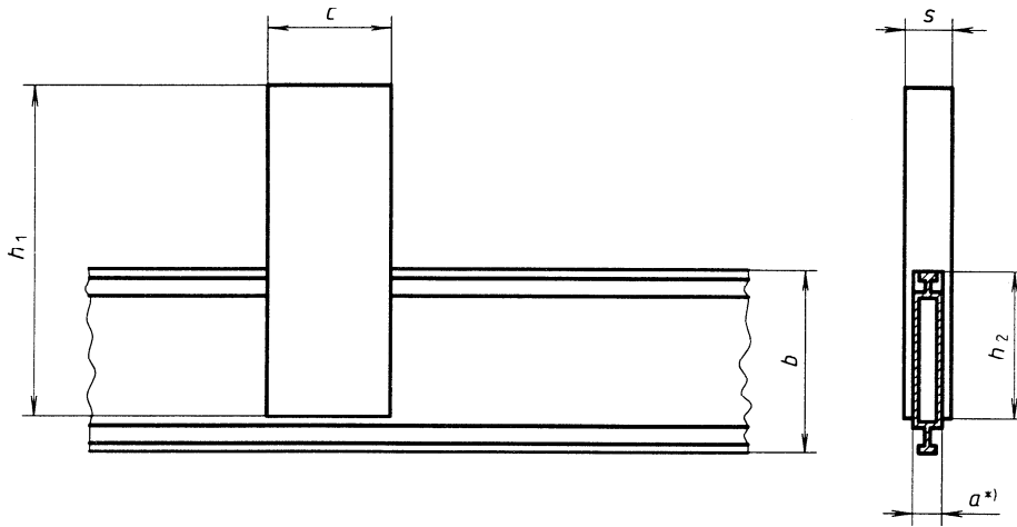
Figure 1 — Heald frame guide
