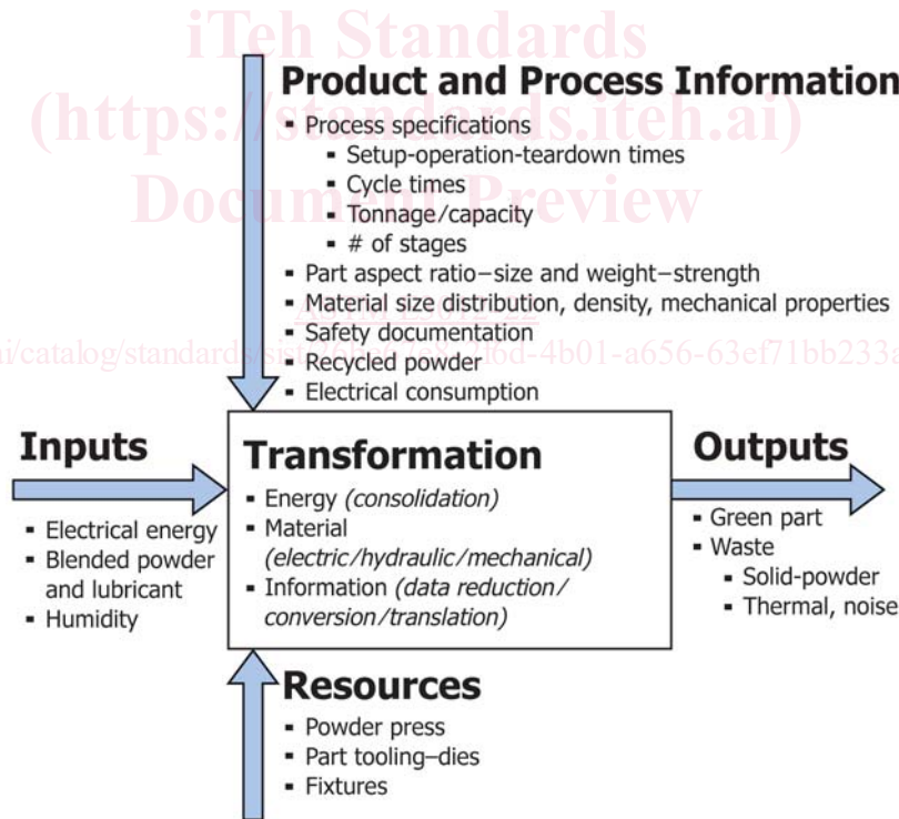
FIG. 5 Graphical Representation of Specific UMP for Compacting Process
