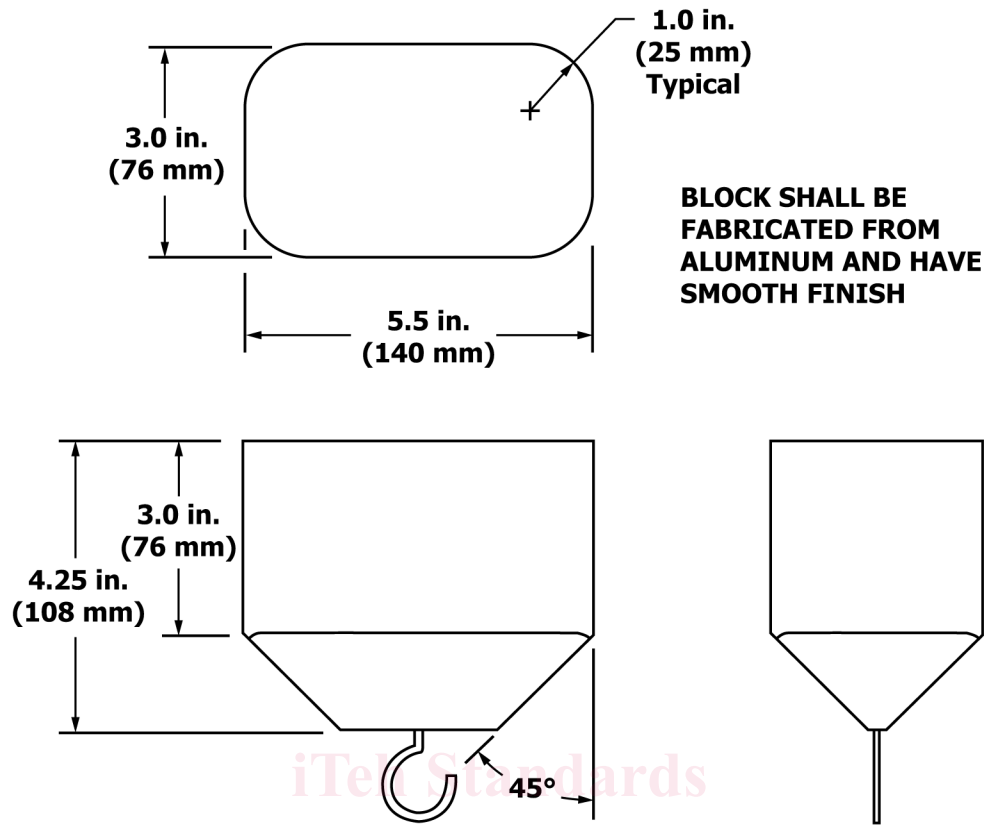
NOTE 1—Not to scale. FIG. 7 Torso Probe
