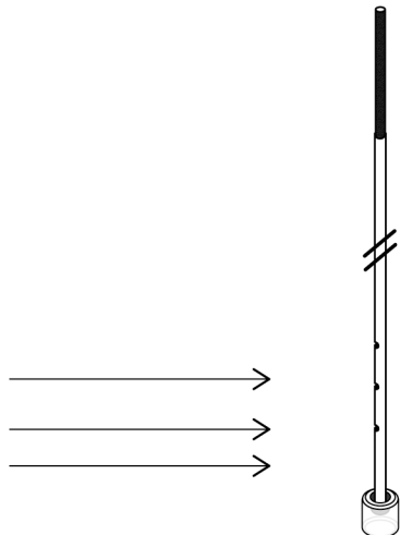
FIG. 5 Example of a Weighted Drop Tube Device
