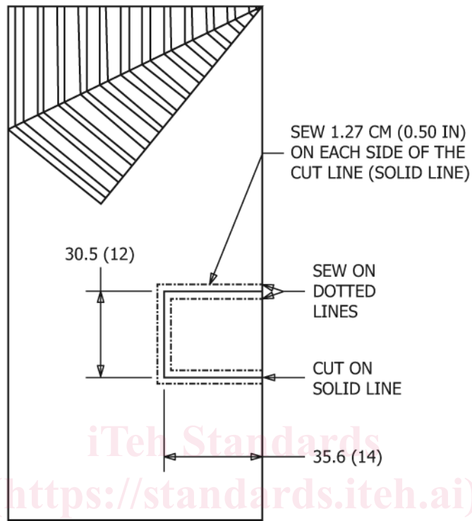
FIG. 1 Test Specimen
