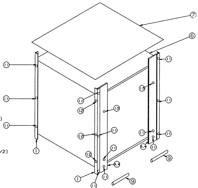
FIG. 2 Test Chamber
