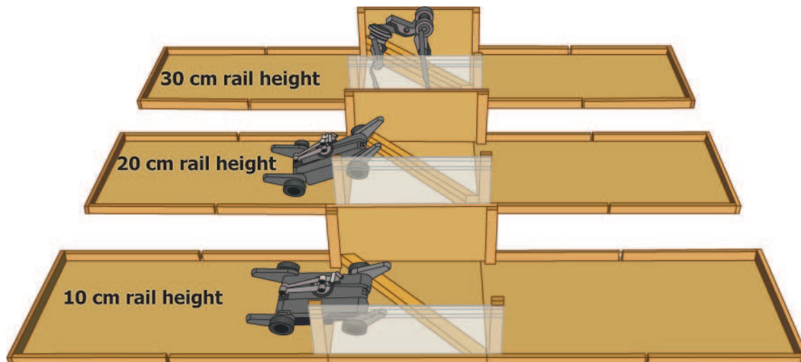
FIG. 1 (A) View of the Variable DiagonalHeight Rail; Shown Heights; Heights: 10 cm [4 in.], 20 cm [8 in.], 30 cm [12 in.]
