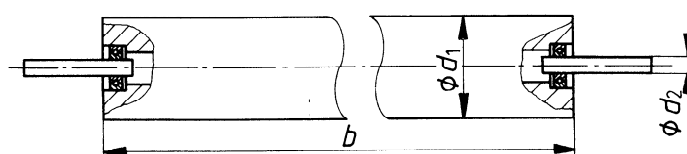
Figure 2 — Type B: Fixed spindle
