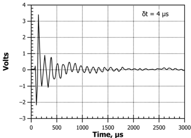
FIG. 5 Waveform and Amplitude Spectrum for Valid Impact-Echo Test of 250-mm Thick Concrete Slab
