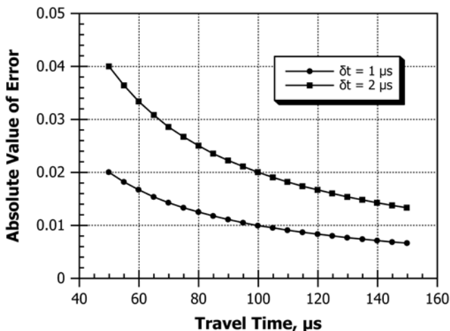
FIG. 7 Maximum Systematic Error Due to Sampling Interval as Function of Travel Time
