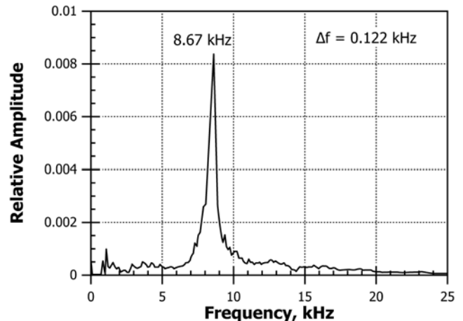
FIG. 5 Waveform and Amplitude Spectrum for Valid Impact-Echo Test of 250-mm Thick Concrete Slab
