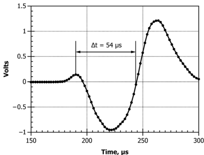
FIG. 3 Expanded View of Surface-Wave Portion of Waveform Showing Width of Surface Wave Signal as Approximation of Contact Time of Impact
