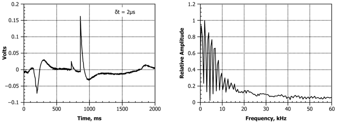
FIG. 6 Example of Invalid Impact-Echo Test, Waveform Does Not Display Periodic Oscillations and Amplitude Spectrum Does Not Have Single Dominant Peak
